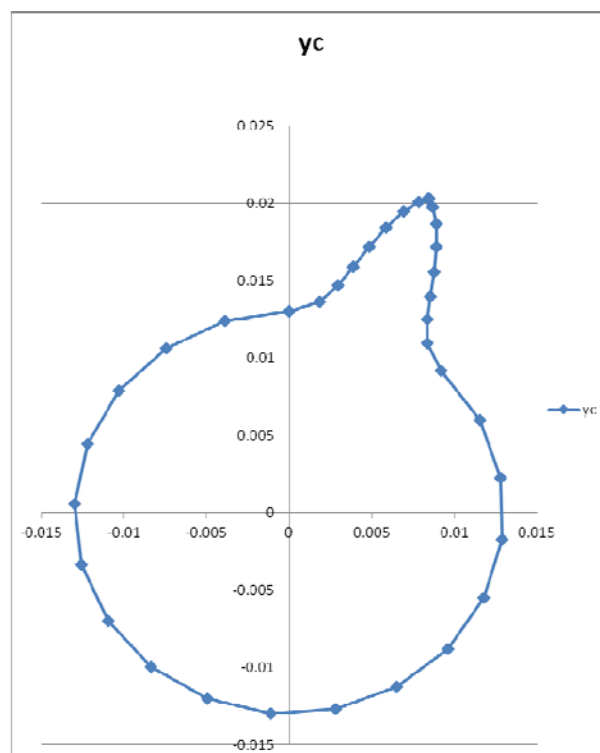
Figure 12: The cosine profile at the cam with translated follower with roll; r_0=13 [mm], h=9 [mm], \varphi_u=\pi/8 [rad], r_b=2 [mm], e=0 [mm].
