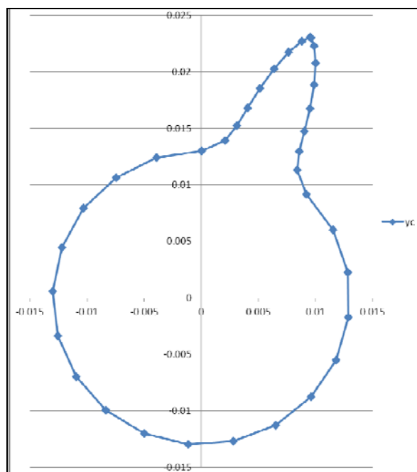
Figure 16: The cosine profile at the cam with translated follower with roll; r_0=13[\text{mm}] , h=12[\text{mm}] , \varphi_u=\pi/8[\text{rad}] , r_b=2[\text{mm}] , e=0[\text{mm}] .
