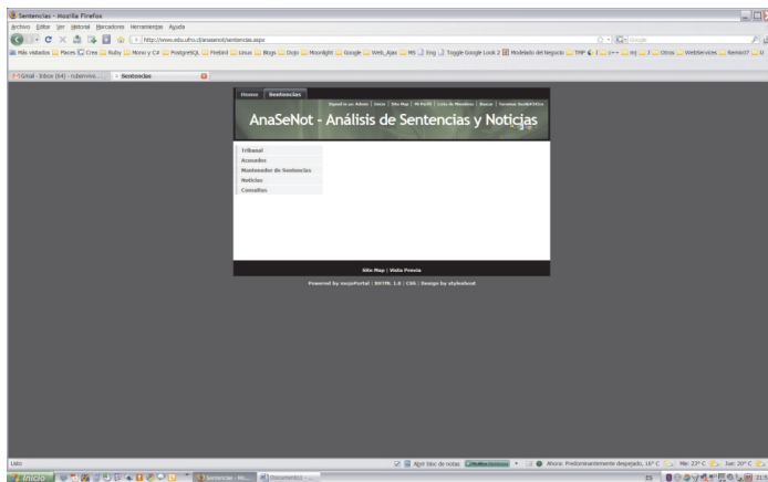
Figura 4. Menú principal
