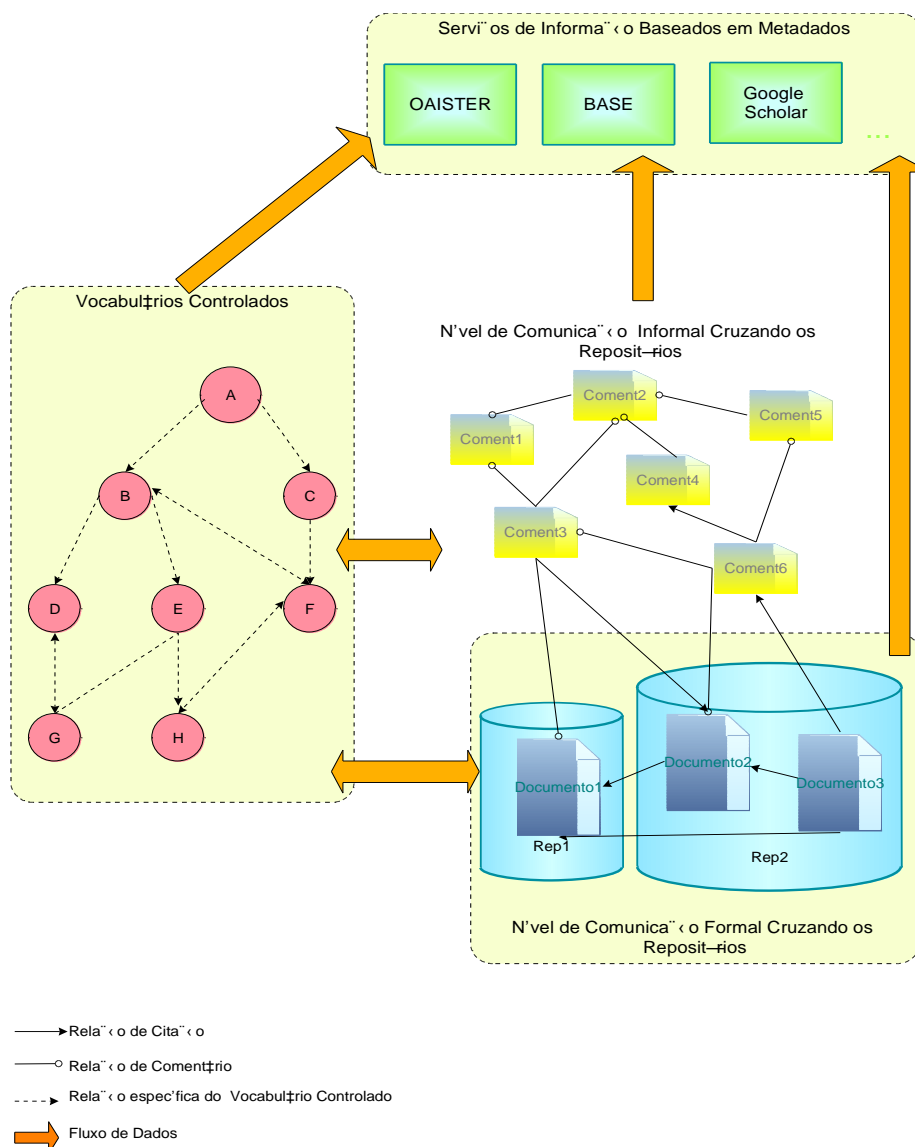
Figure 4 - Architecture of the new comment service.
