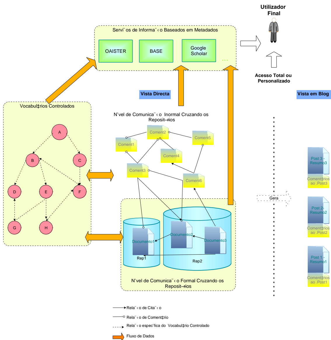
Figure 5 – Final architecture of the new comment system
